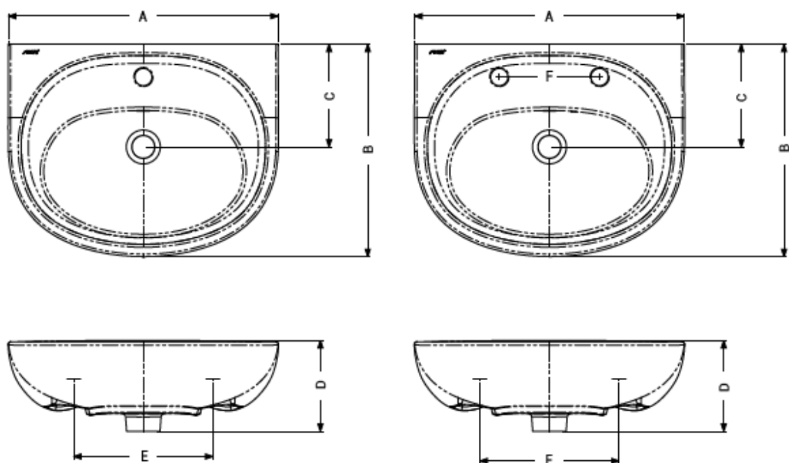
550mm wash basin
