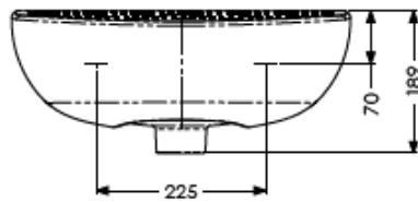
Navlin 450mm Wash Basin One Tap Hole
