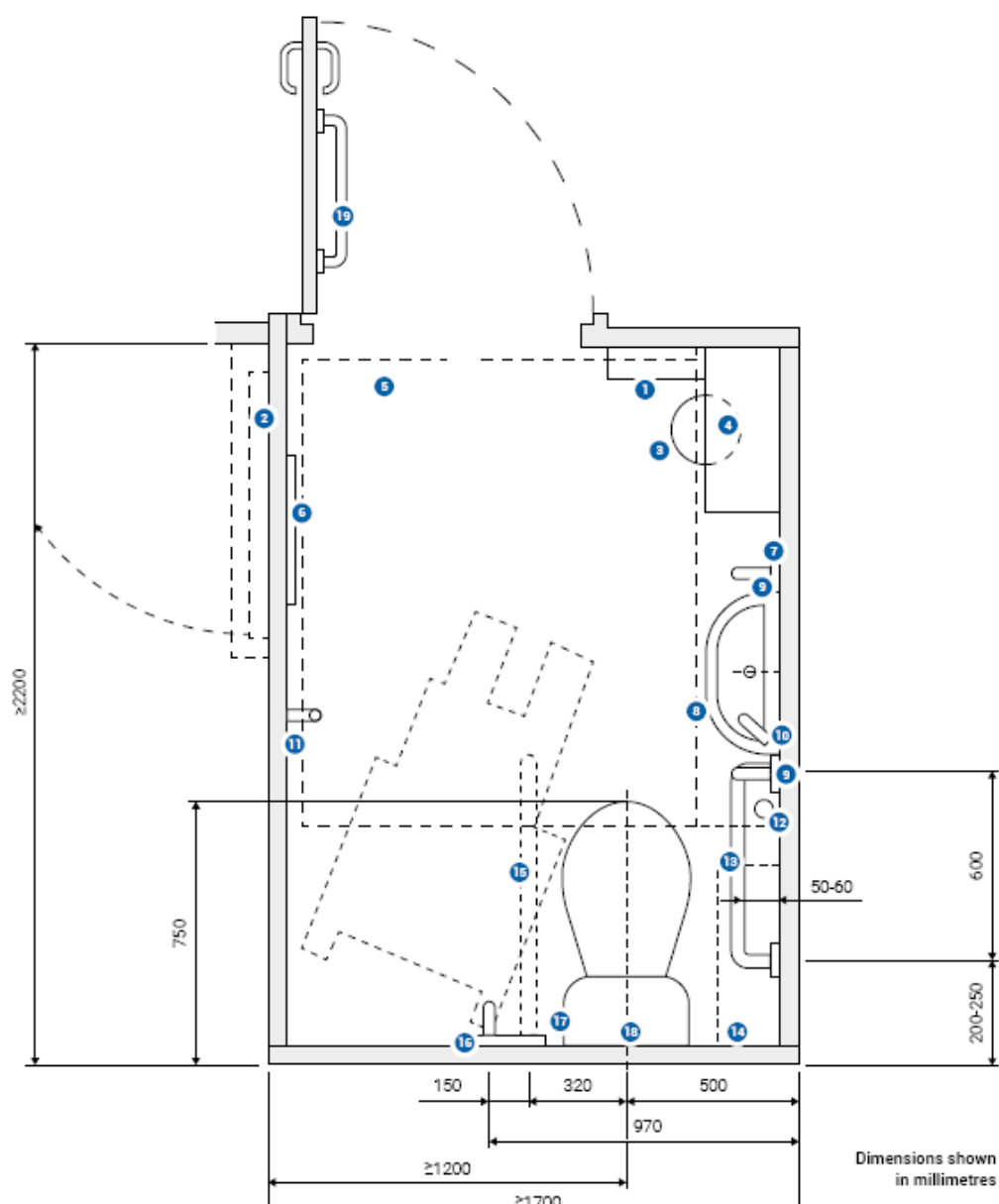
Plan View
