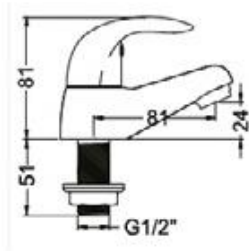
AKW Denova Wash Basin Taps Dimensions
