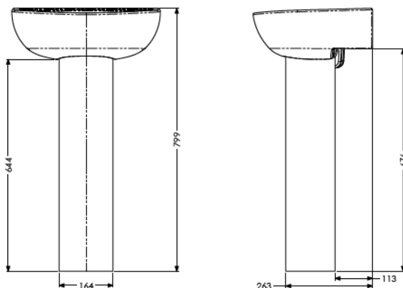
Navlin 450mm Wash Basin with Full Pedestal
