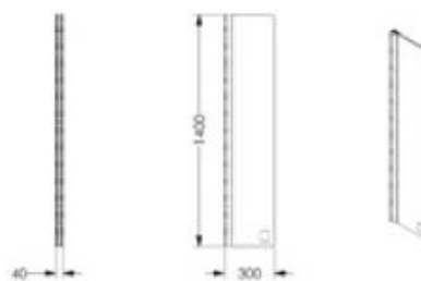
Fixed Square Top Bath Shower Screen 300mm
