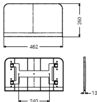
Onyx Seat Back and Arms – Back Rest
