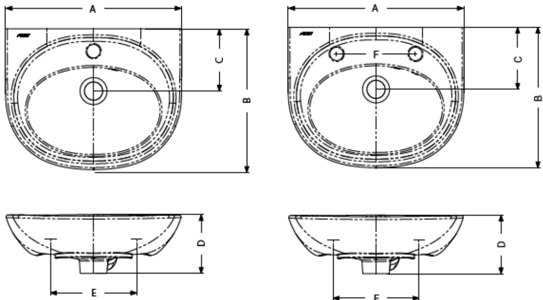
450mm wash basin
