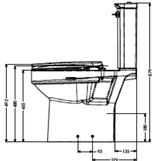
Navlin Doc M Raised-Height Close-Coupled Toilet Pan (650mm), Cistern with Lever Flush and Ergonomic Seat & Lid
