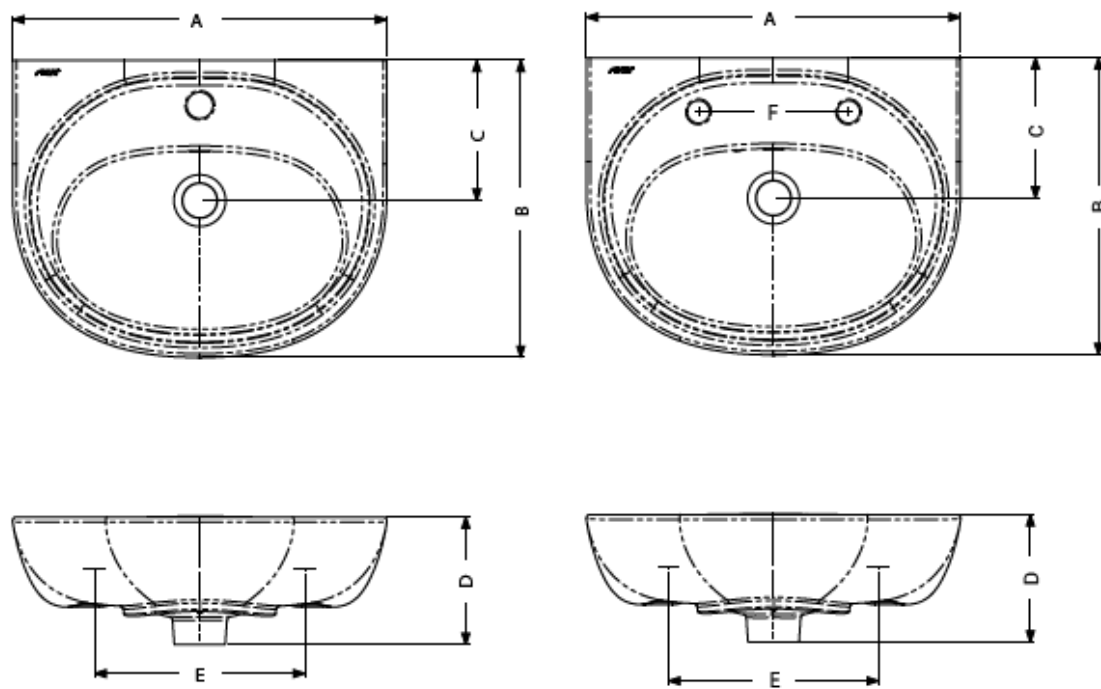
500mm wash basin
