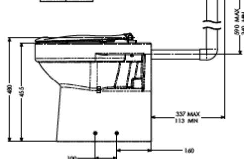
Navlin Doc M Low-Level WC with Lever Flush & Flush Pipe
