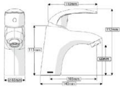
AKW Denova Basin Mono Mixer Tap Dimensions
