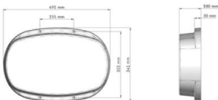
100mm High SMC Toilet Plinth
