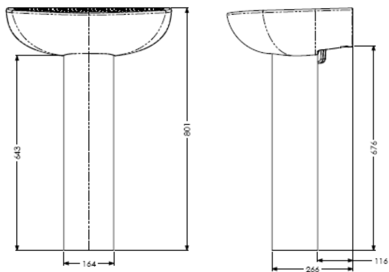
Navlin 550mm Wash Basin with Full Pedestal
