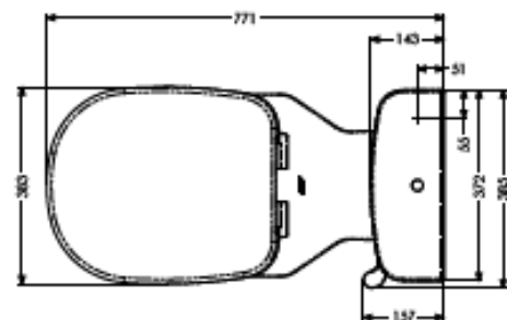
Navlin Doc M Raised-Height Close-Coupled Toilet Pan (650mm), Cistern with Lever Flush and Ergonomic Seat & Lid
