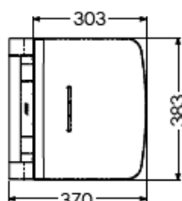
Onyx Compact Fold-Up shower Seat
