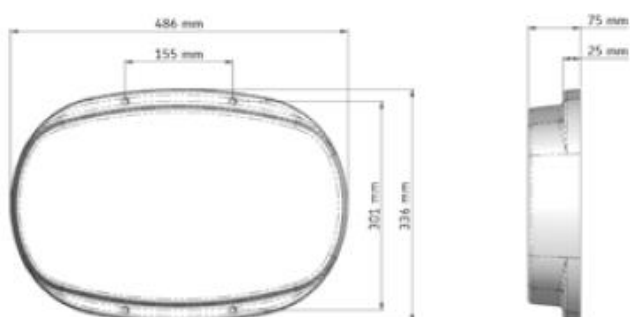
75mm High SMC Toilet Plinth
