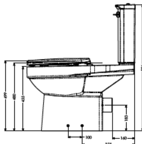
Navlin Doc M Raised-Height Close-Coupled Toilet Pan (750mm), Cistern with Lever Flush and Ergonomic Seat & Lid
