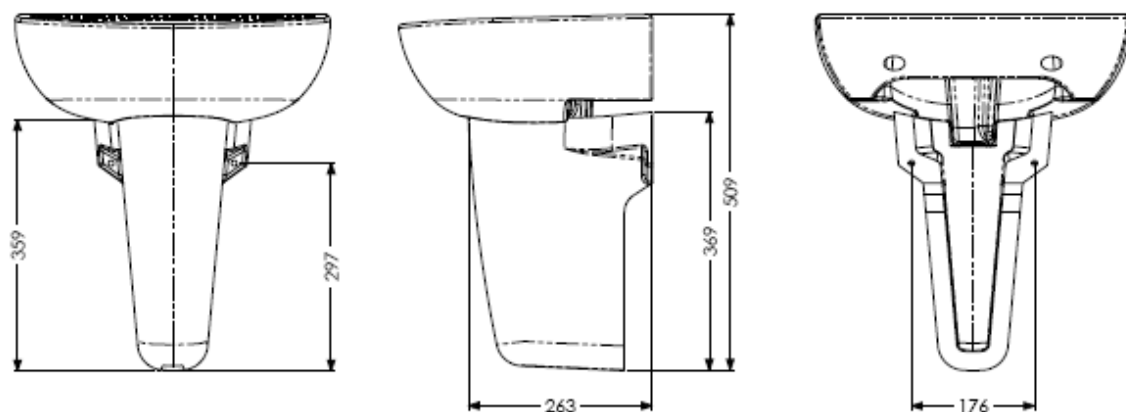
Navlin 450mm Wash Basin with Semi Pedestal
