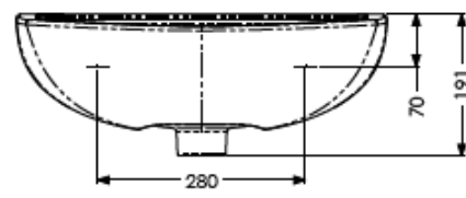
Navlin 500mm Wash Basin Two Tap Holes
