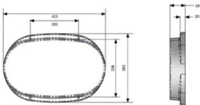
59mm High GRP Toilet Plinth
