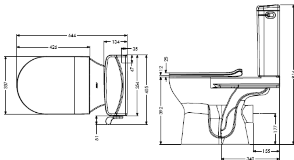
Livenza Plus close-coupled WC with lever flush
