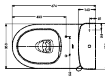
Navlin Raised-Height Close-Coupled Toilet Pan & Cistern with Raised Push Button Flush
