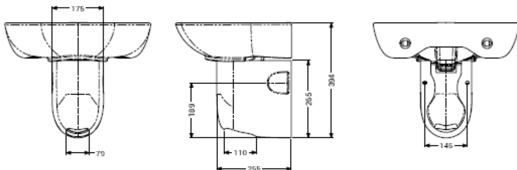
Semi pedestal for 500mm wash basin
