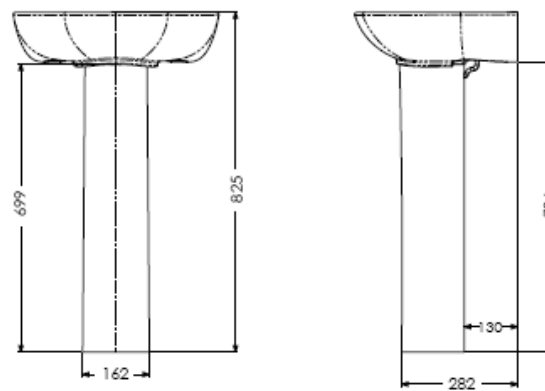
Full pedestal for 500mm wash basin
