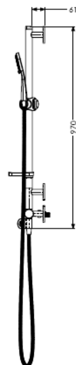
Onyx Combo Mixer Shower LH
