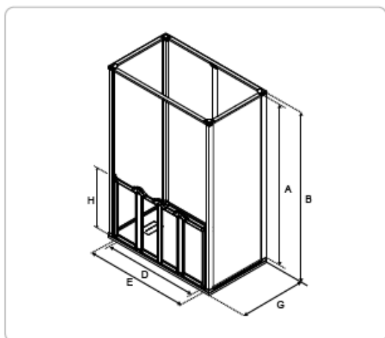
Alcove / Corner Option N (Fig 5)
