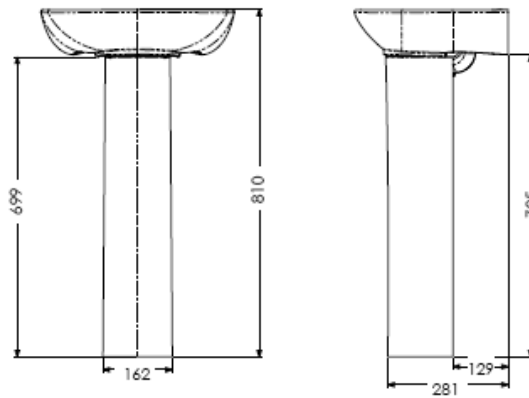
Full pedestal for 450mm wash basin
