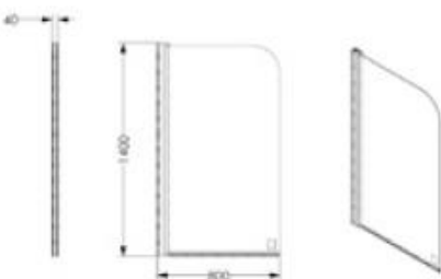
Hinged Curved Top Bath Shower Screen 800mm
