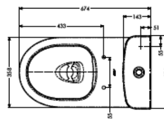
Navlin Standard-Height Close-Coupled Toilet Pan & Cistern with Raised Push Button Flush
