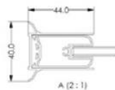
Fixed Shower Screen Profile
