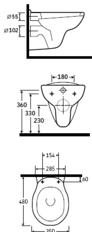
Dimensions (mm)
