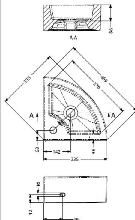
Dimension (mm)
