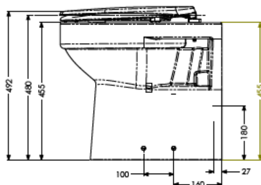
Navlin Doc M Back-to-wall Toilet Pan with Ergonomic Seat & Lid
