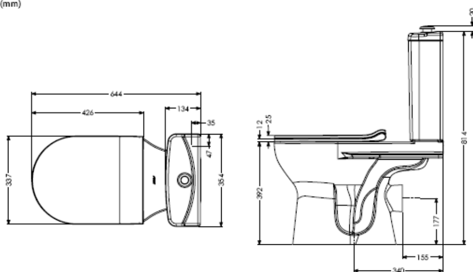
Livenza Plus close-coupled WC with raised push button flush
