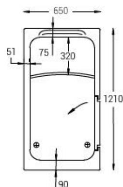
Dimensions (mm)
