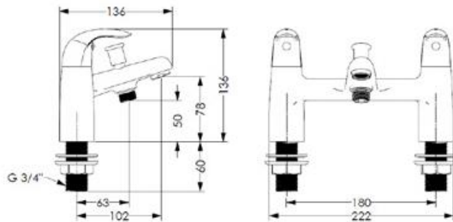
AKW Denova Bath Shower Mixer Taps Dimensions
