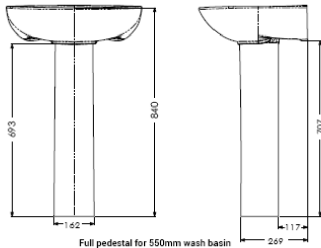
Full pedestal for 550mm wash basin
