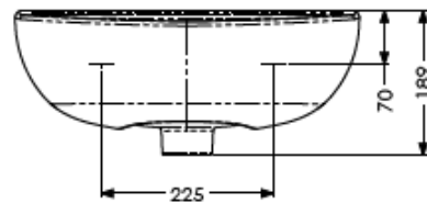
Navlin 450mm Wash Basin Two Tap Holes
