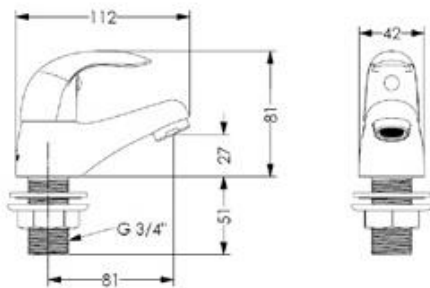
AKW Denova Lever Bath Taps Dimensions
