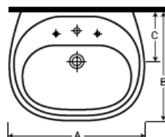
Dimensions (mm)
