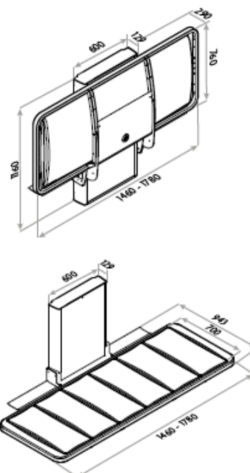
Dimensions (mm)
