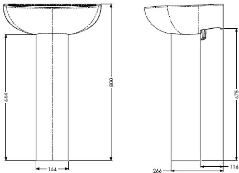
Navlin 500mm Wash Basin with Full Pedestal
