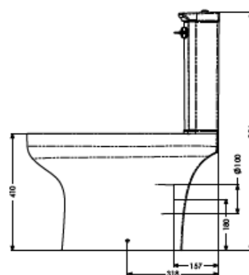
Navlin Standard-Height Close-Coupled Toilet Pan & Cistern with Raised Push Button Flush
