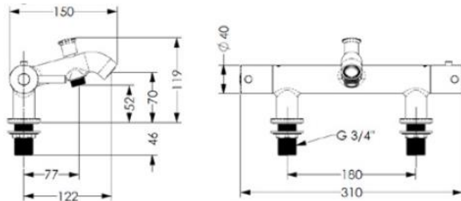
Thermostatic Peg Lever Bath Shower Mixer Tap
