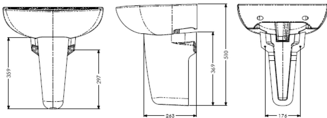
Navlin 500mm Wash Basin with Semi Pedestal
