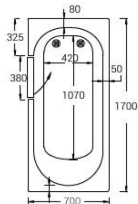
Dimensions (mm)
